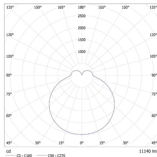
Lucis ZL4.IR.L11.700M.1 IZAR R MAX LED / LDC (Polar)
